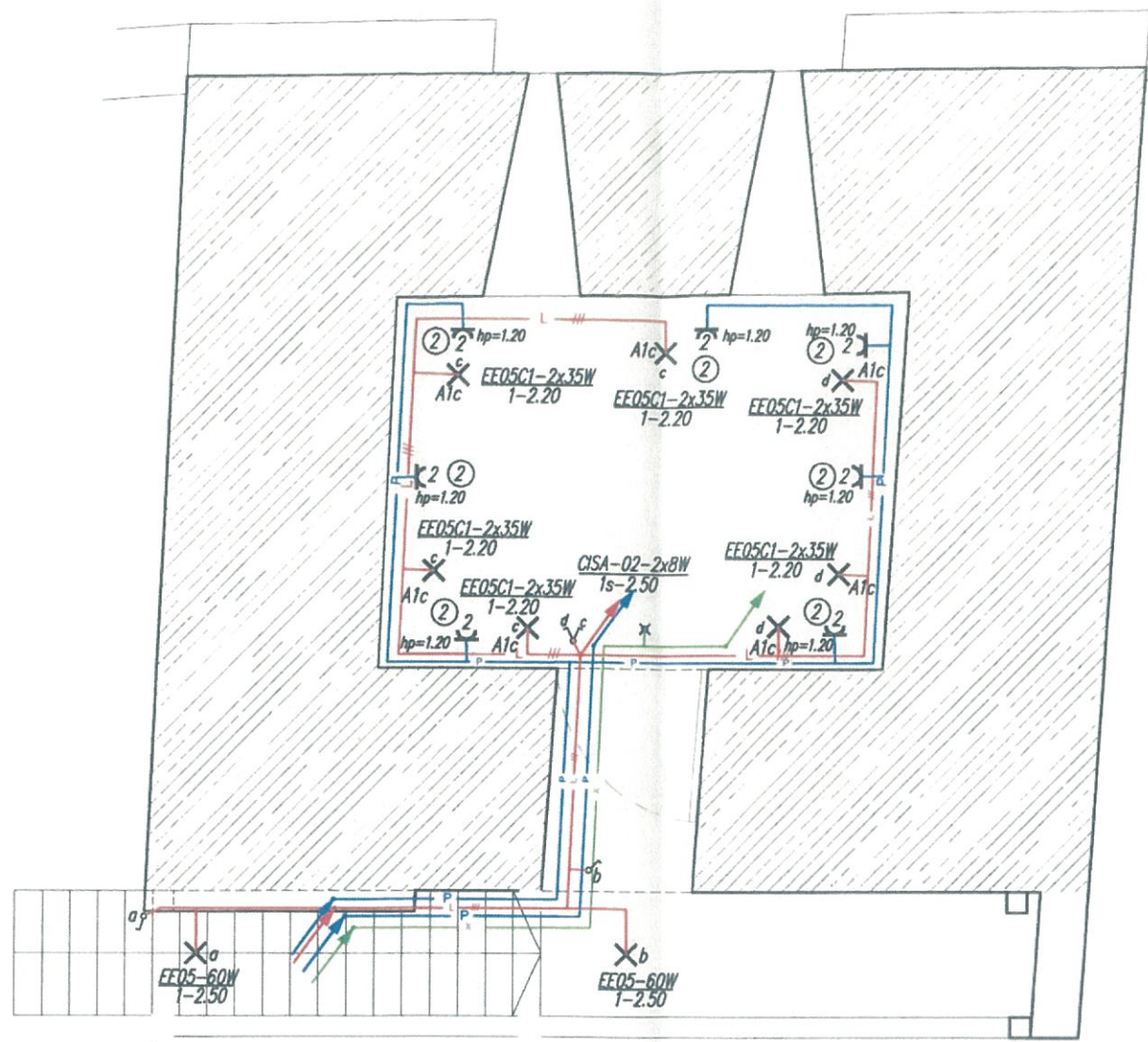
Plan cota +5.80
