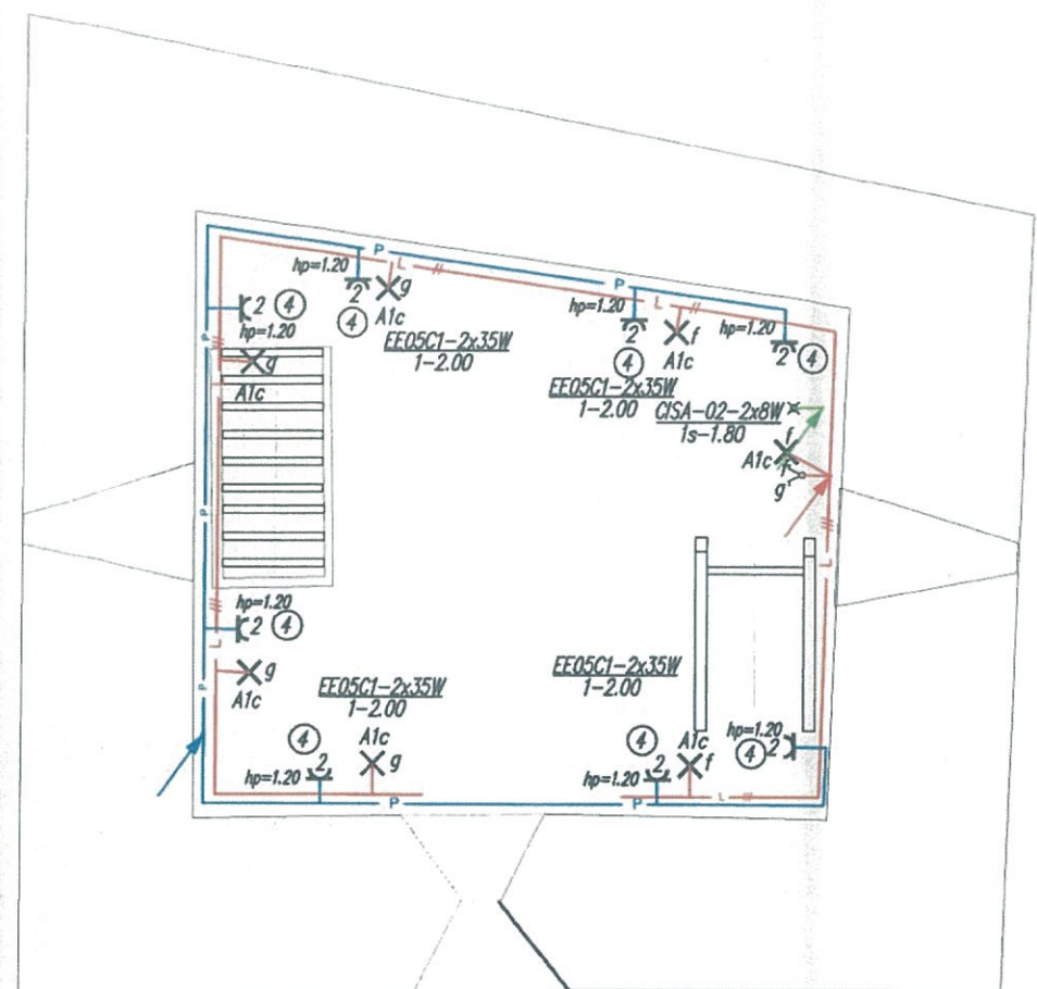
Plan cota +5.00m
