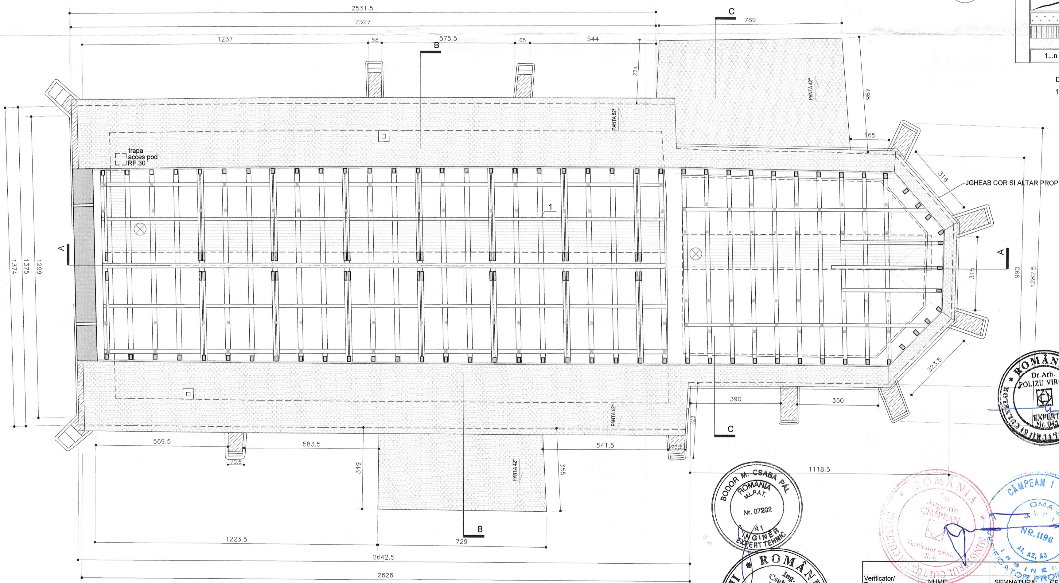
PLAN POD
