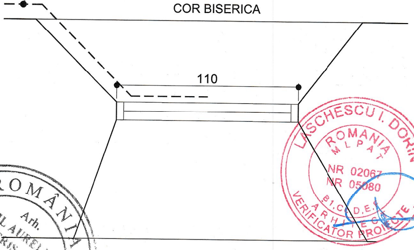
PLAN SCARA 1/20
